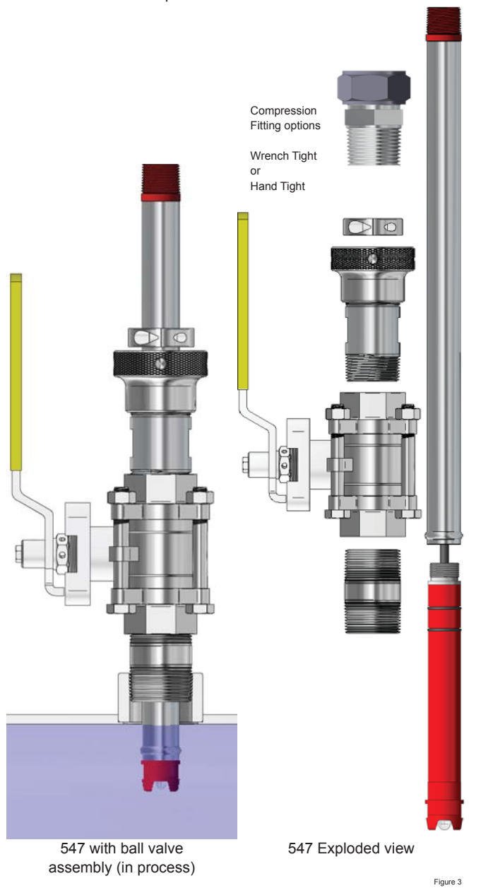
547 Retractable “Hot Tap” Sensors
