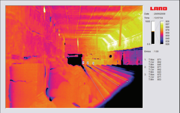
Temperature Profiles inside the furnace
