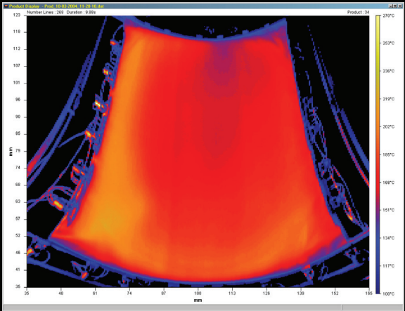
Uncorrected thermal map of heated plastics sheet exiting a rotary thermoforming machine
