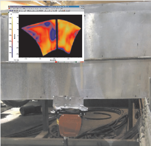
Scanner mounted below the sheet on a thermoforming machine. Inset shows typical thermal profile before correction.
