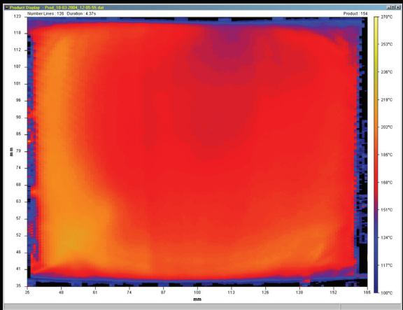
Thermal profile after correction applied by the Landscan Thermoforming software
