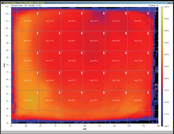
Corrected thermal profile with over lay of heater zones
