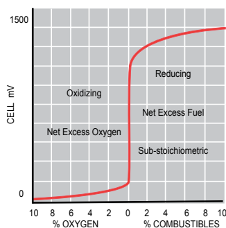
Zirconia cell output for Excess Oxygen and Excess Fuel
