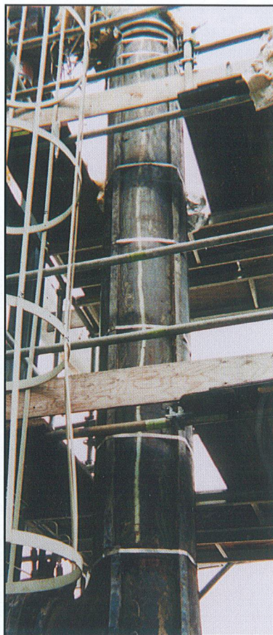
The sulfur pipeline at an Alberta, Canada, natural gas plant has been operational for one and a half years since installation of new bolt-on heat trace elements.
