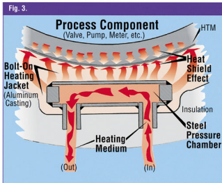
Fig. 3. The primary function of the bolt-on heat jacket is to act as a heat shield, compensating for process heat loss during normal operation.
