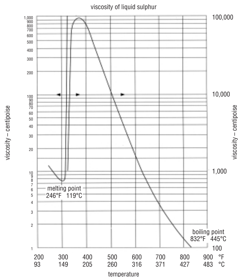
Fig. 1: Viscosity of liquid sulphur
