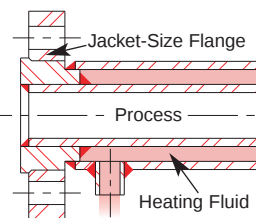
Non-Reducing Insert Flange
