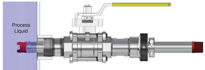
547 Retractable "Hot Tap" pH Sensor with Isolation Ball Valve
